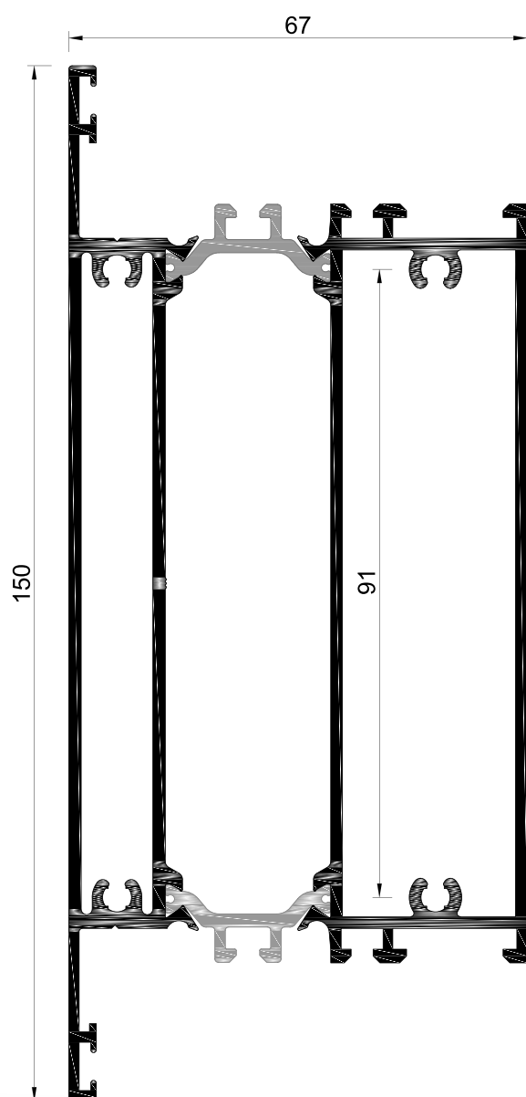
LT.14 Travessa Central / Inferior
