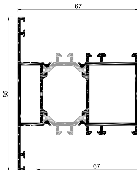
LT.36 Travessa
