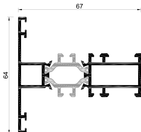
LT.14 Travessa Central / Inferior
