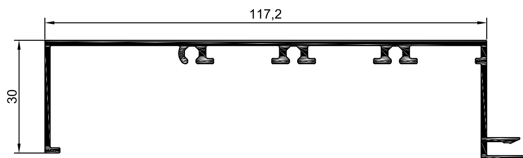
AQ.160 Remate
