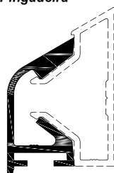
SA.32 Pingadeira
