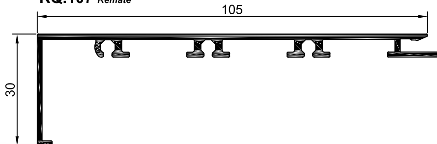
RQ.107 Remate
