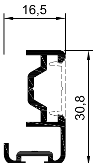
POC.11 Remate Lateral (Mono-Rail)
